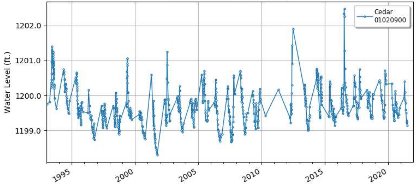
Recorded Water Levels 1993-01-01 to 2021-12-31
