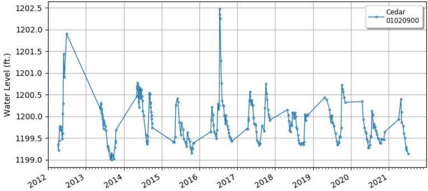
Recorded Water Levels 2012-01-01 to 2021-12-31
